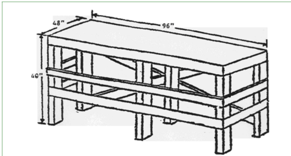
FIGURE 2-1 Diagram of a General Inspection Table
